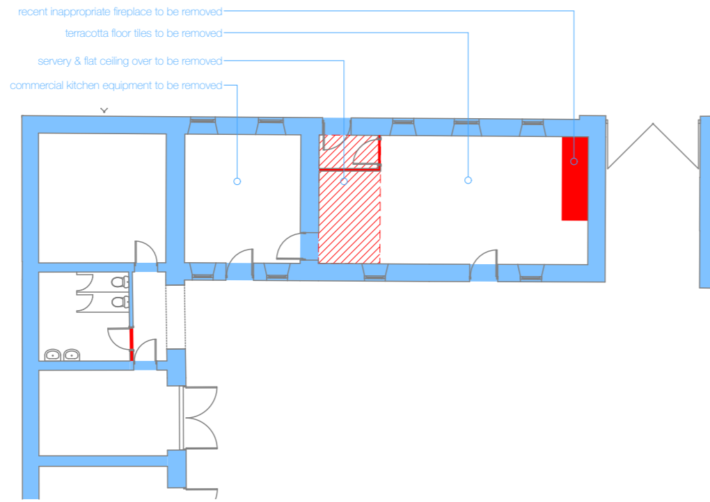
0. Conservation Demolition Ground Floor 1:200
